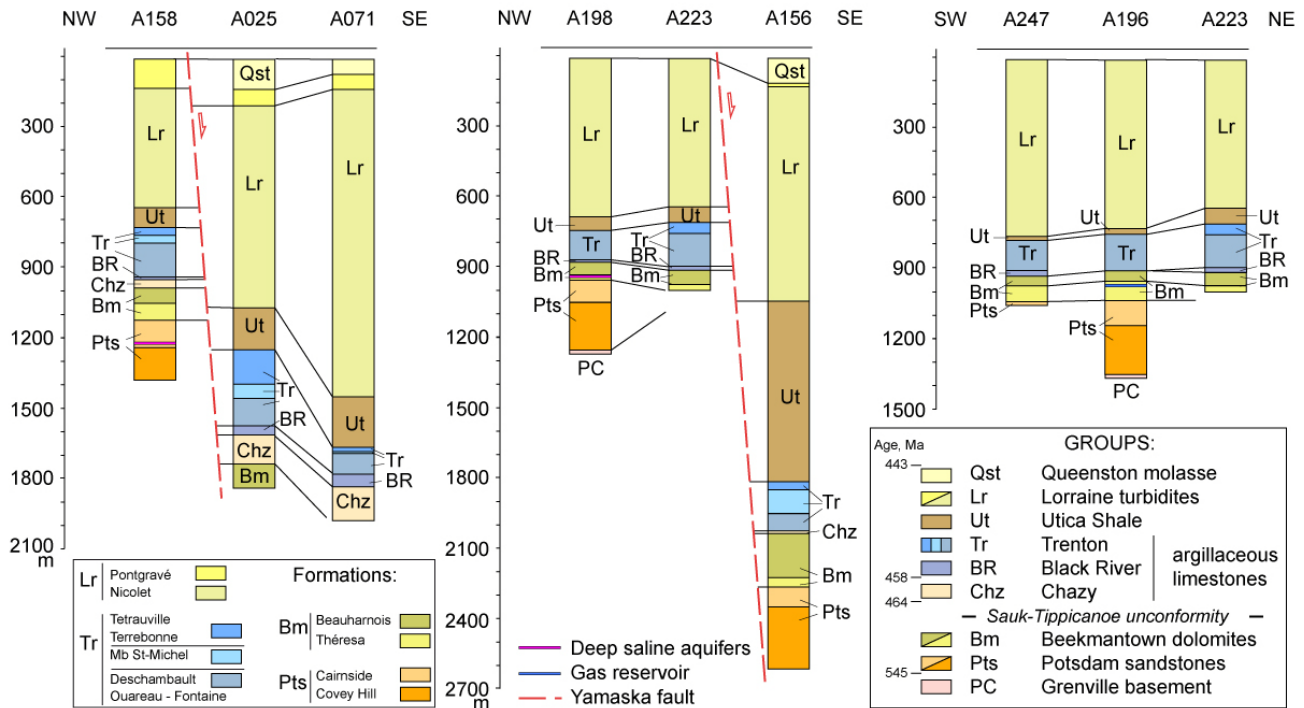
Fig. 2. Lithostratigraphic correlations of the St. Lawrence Lowlands successions based on well data reports from the MRNF Quebec database. The location of wells is given in Fig. 1.
