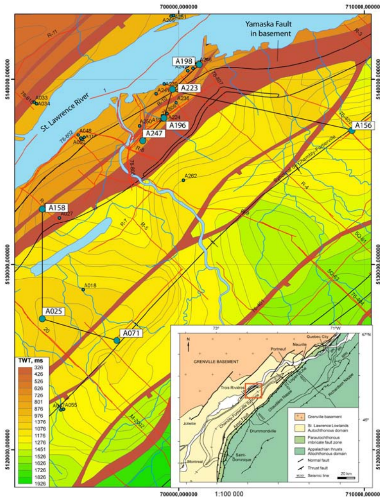
Fig. 1. Map of the Grenvillian basement in the Bécancour area, Quebec, after Thériault et al. (2005). Location of wells at Fig. 2 is shown. Red lines are available seismic profiles.
